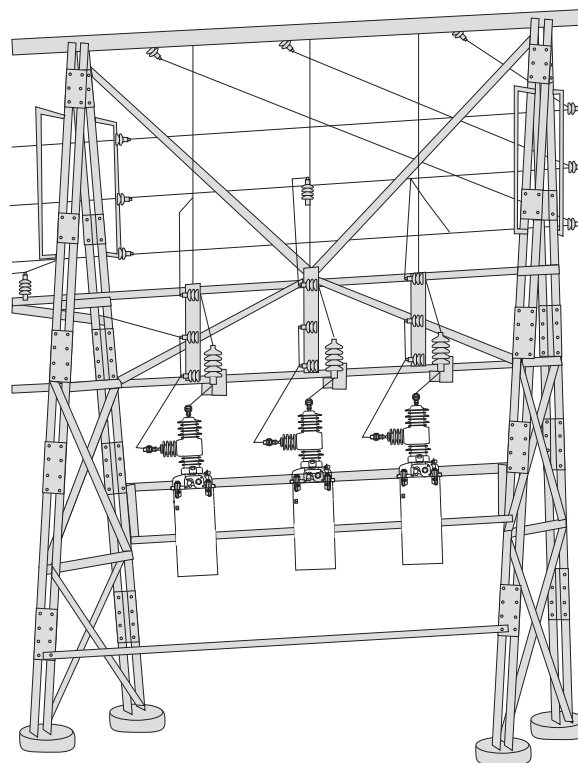
Figure 6. Substation mounting.
