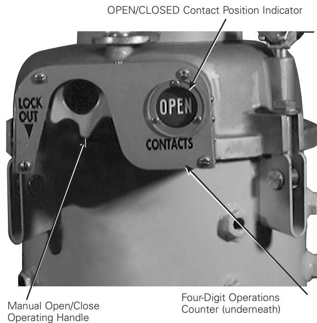
Figure 10. NOVA-TS triple-single recloser operating levers and indicators.
